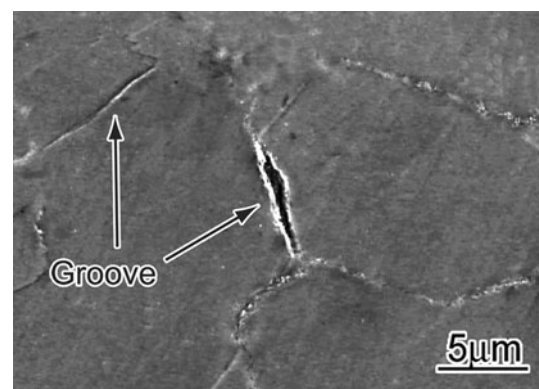
Fig. 5 SEM image showing the surface appearance after a 40° W-shape bending test of a Cu–1.8% Be–0.21% Co alloy aged at 320 °C for 30 min
