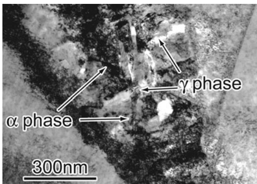
Fig. 7 TEM image of a DP cell in a Cu–1.8% Be–0.21% Co alloy rolled to 10% reduction after aging at 320 °C for 30 min
