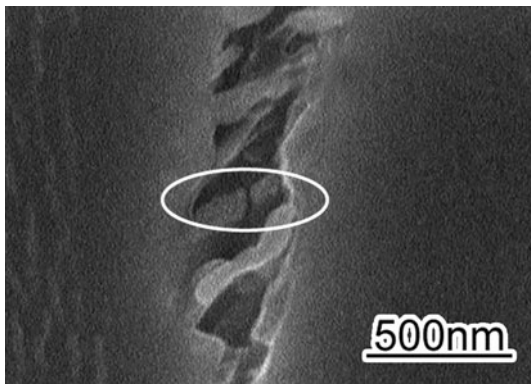
Fig. 6 SEM image of a void formed by destruction of a \gamma precipitate in a DP cell after a 20° W-shape bending test and subsequent etching of a Cu–1.8% Be–0.21% Co alloy aged at 320 °C for 30 min
