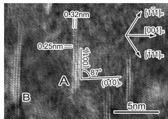
Fig. 1 HRTEM image of \gamma'_1 precipitates in a Cu–1.8 wt% Be–0.21 wt% Co alloy aged at 320 °C for 30 min. The zone axis is parallel to [110]_\alpha
