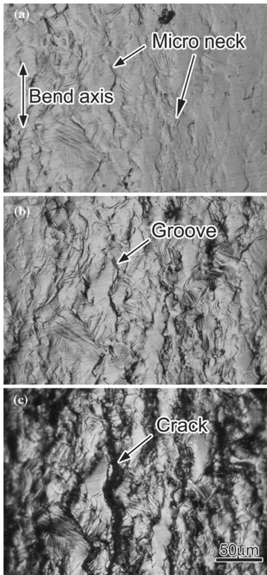
Fig. 4 Optical microscopy images showing the surface appearances of the same area after a 20°, b 40° and c 60° W-shape bending tests of a Cu–1.8% Be–0.21% Co alloy aged at 320 °C for 30 min
