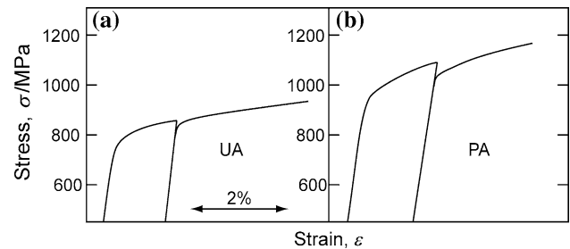
Fig. 3 Stress–strain curves before and after annealing at 200 °C for 3 h for Cu–1.8% Be–0.21% Co specimens aged at 320 °C for 30 min (UA) and for 3 h (PA)
