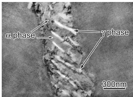
Fig. 2 TEM image of a DP cell in a Cu–1.8% Be–0.21% Co alloy aged at 320 °C for 30 min
